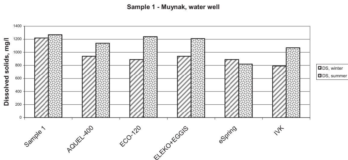
Figure1: The changes of the content of dissolved solids in the sample 1 after the treatment by different types of water cleaning devices
