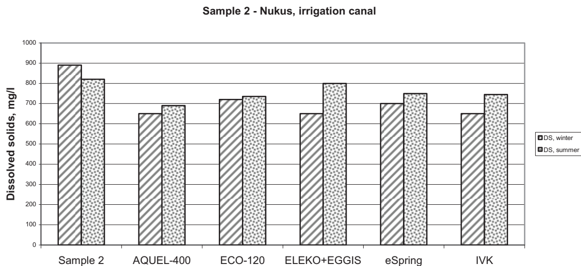
Figure 2: The changes of the content of dissolved solids in the sample 2 after the treatment by different types of water cleaning devices.
