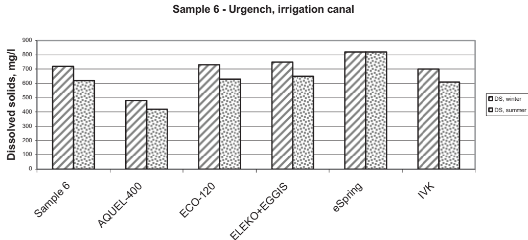
Figure 6: The changes of the content of dissolved solids in the sample 6 after the treatment by different types of water cleaning devices
